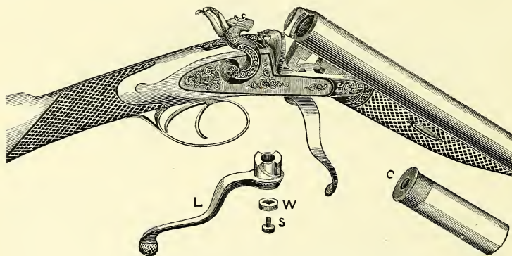
The Double-grip Bar-lock Gun, and Central-fire Cartridge.
